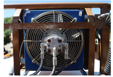
OIL COOLER
